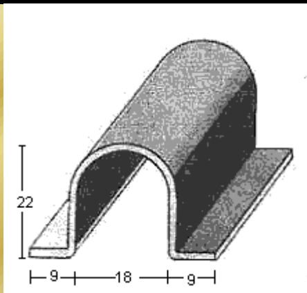
1521 (1,5mm.)
